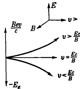
FIG. 1-22.—Paths of electrons in crossed electric and magnetic fields.
